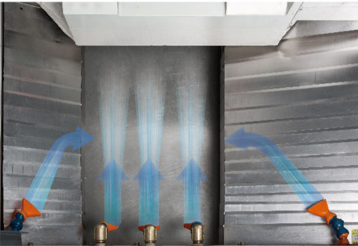
Widely slanted sheet metal with central chip disposal device allows chips efficient removing efficiently.
